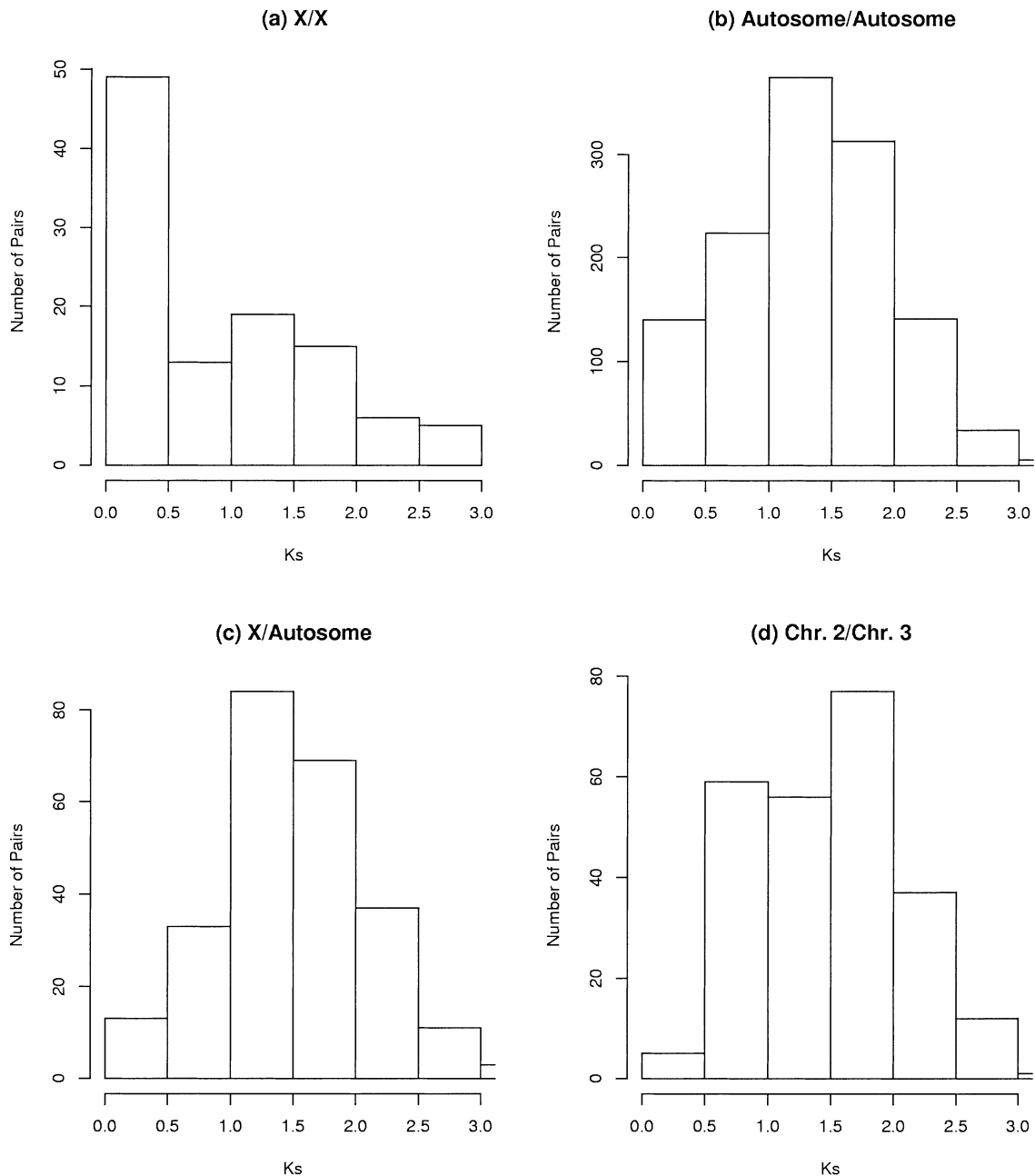
FIG. 2.—Frequency distributions of K_s between paralogous genes in D. melanogaster . a , The distribution of K_s between duplicates on the X chromosome, showing a large fraction of pairs with low K_s . b , The distribution of K_s for linked, autosomal duplicate pairs. c , The distribution of K_s for X-autosome duplications. d , The distribution of K_s for duplications between chromosomes 2 and 3.
