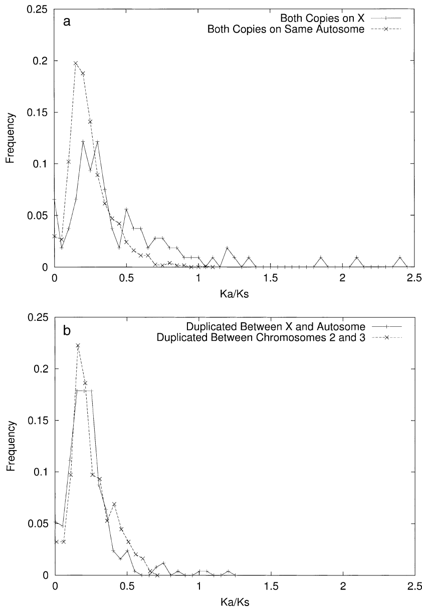
FIG. 1.—Frequency distributions of K_a/K_s between paralogous genes in D. melanogaster . K_a/K_s is binned into groups of size 0.05. a , The distribution of K_a/K_s between duplicates on the same chromosome. The distribution for X-to-X duplicates shows a long tail to the right and a higher mean value (table 1) than duplicates both linked to the same autosome. b , The distribution of K_a/K_s for unlinked duplicates, i.e., between the X and an autosome or between chromosomes 2 and 3, the major autosomes of D. melanogaster . Compared with ( a ), the two distributions plotted look nearly identical, with the exception of a small tail to the right (indicating rapidly diverging genes) for X-autosome duplicates.
